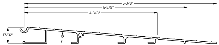
XXXXW - 6-3/8" EXTENDER WITH BREAK POINTS SHOWN
